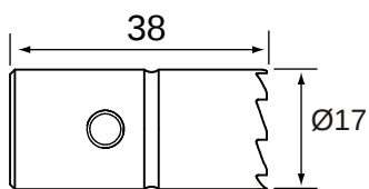
17 x 17 mm flat reamer
