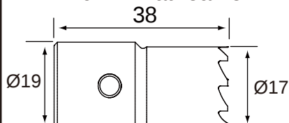
17 x 19 mm flat reamer
