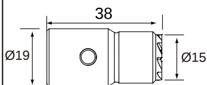
15 x 19 mm flat reamer
