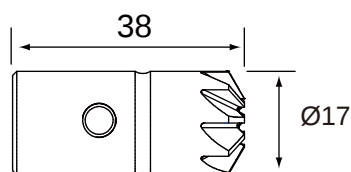
17 x 17 mm angled reamer
