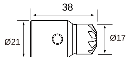
17 x 21 mm angled reamer
